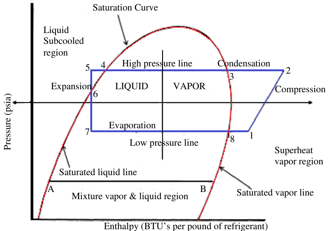
Figure 2. Basic Refrigeration Cycle.
