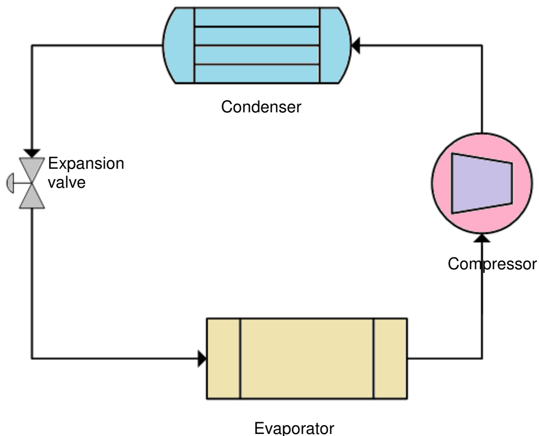
Figure 1. Components of a Refrigeration system.
