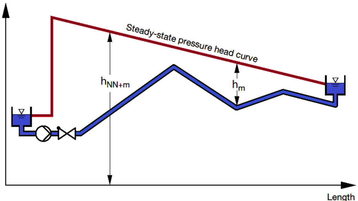
Figure 2: Steady-state pressure head curve of a pumping system
