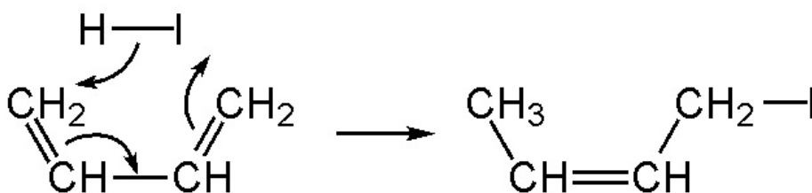
Figure 5. The addition of HI.
