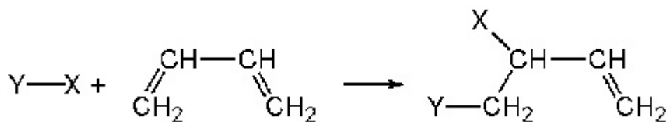
Figure 2. 1,2-addition product
