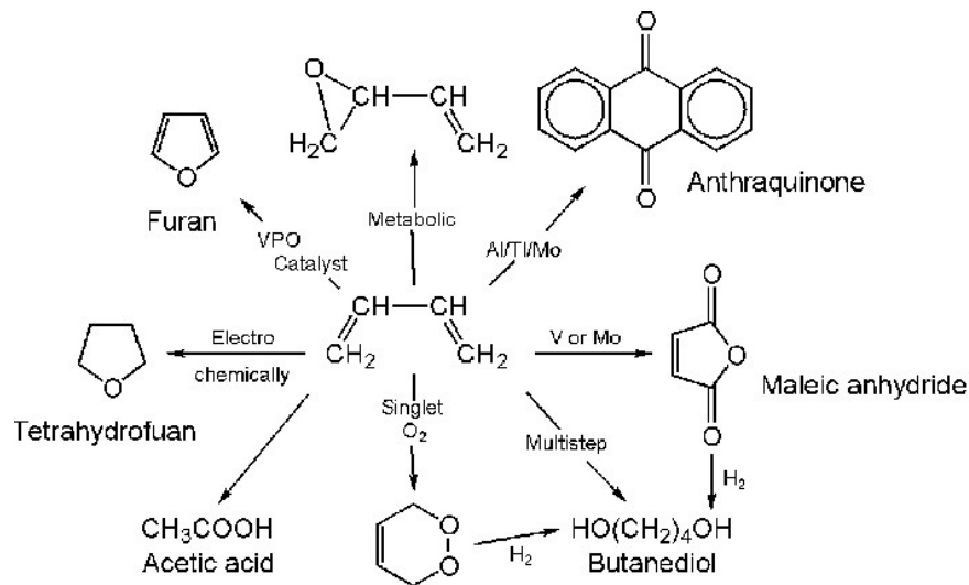
Figure 12. Oxidized products of butadiene.
