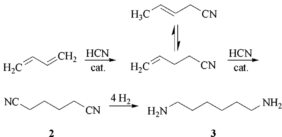
Figure 6. The addition of HCN
