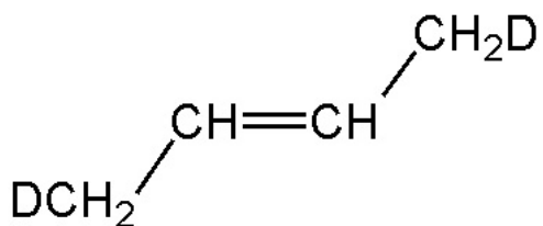
Figure 11. Trans -2-butene-d 2
