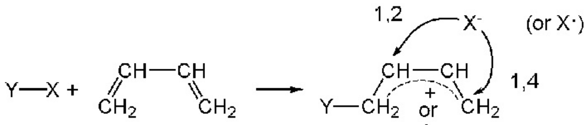
Figure 4. The intermediate of addition product.
