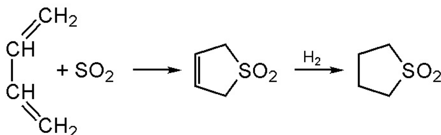
Figure 9. Addition of \text{SO}_2
