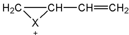
Figure 7. 1,2-cyclic intermediate
